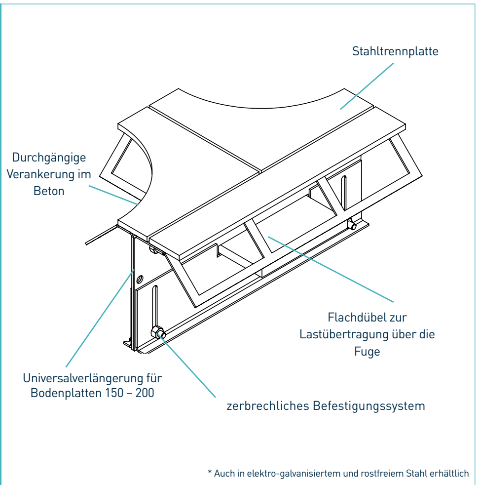
Permaban Wave® T-Section
