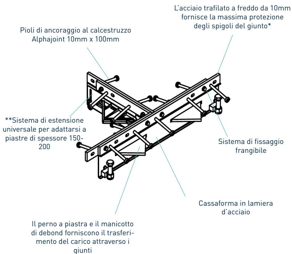
Alpha® 4010 T-Section
