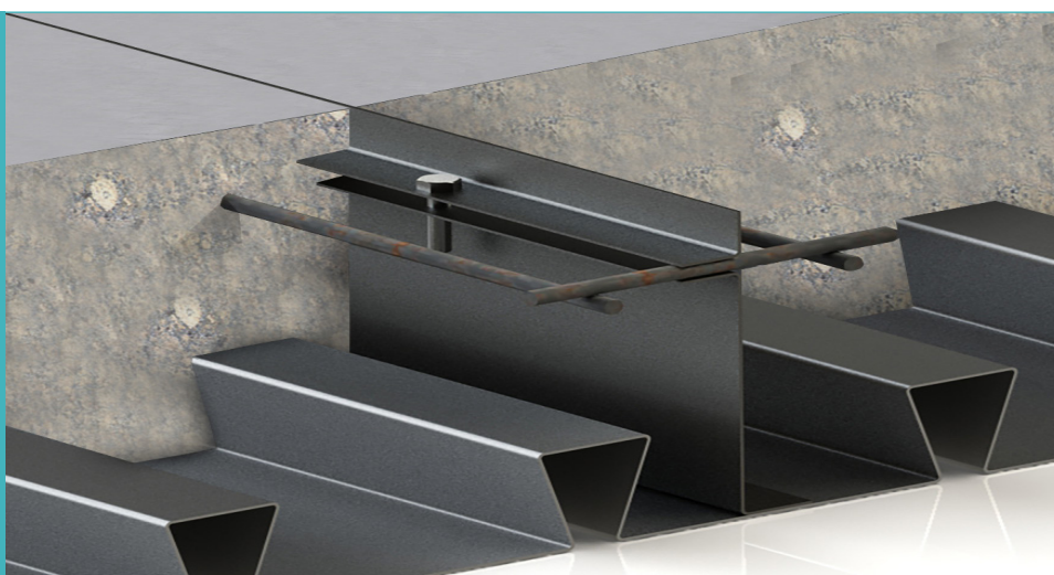
Permadeck Type 1® Surco
