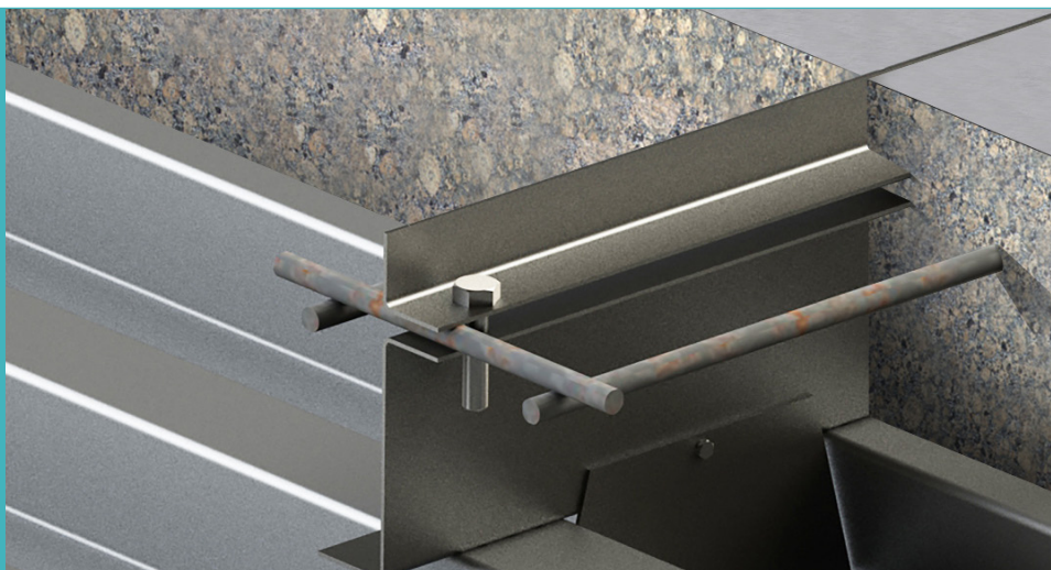
Permadeck Type 1® Perpendicular
