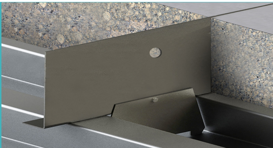
Permadeck Type 2® Perpendicular
