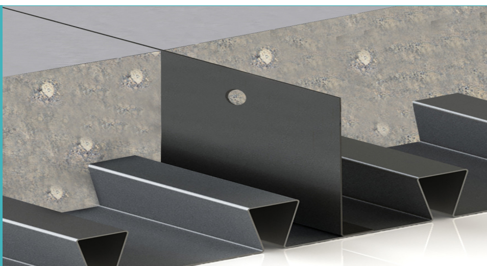
Permadeck Type 2® Surco
